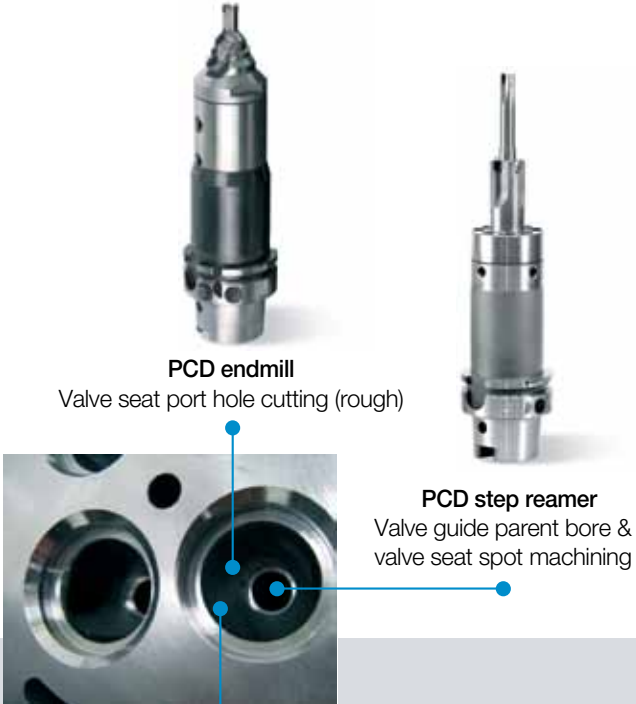
PCD reamer Valve guide reaming
